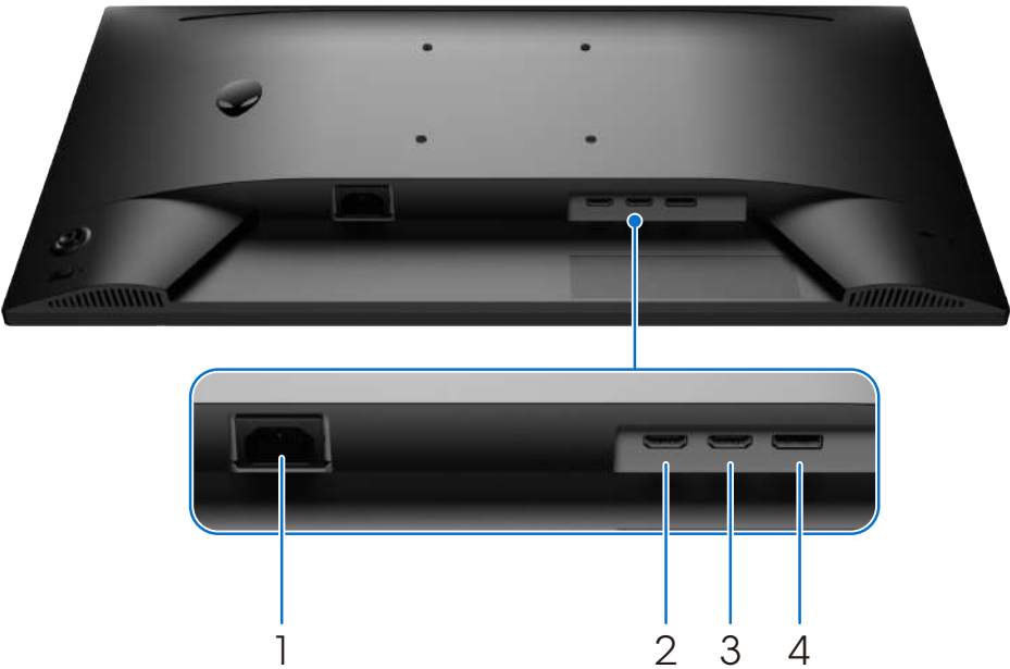
Figure 4. Bottom view of the monitor (AW2526HL)
